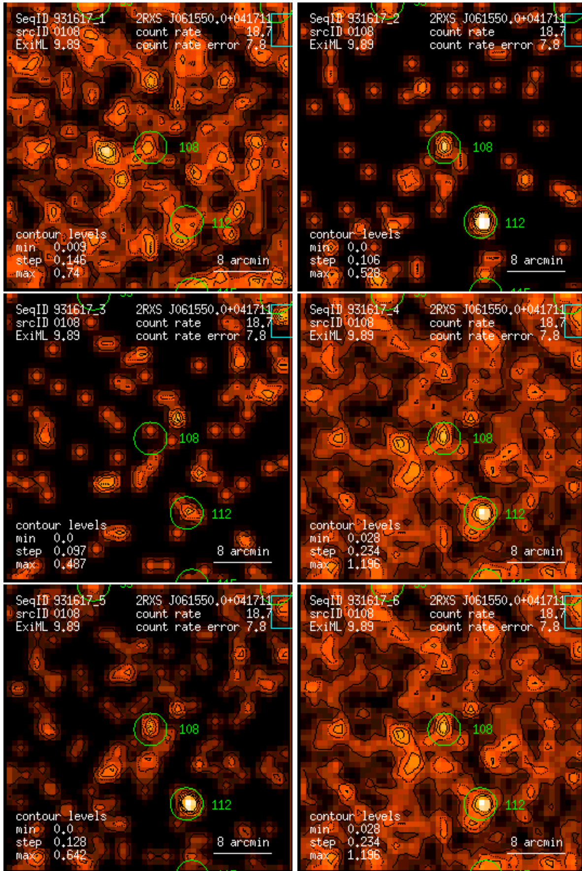
Figure 108: RASS 931617: detection 0108: band rate images, Gaussian filter: (1) PSPC channels 11 – 41, (2) 52 – 90, (3) 91 – 201, (4) 11 – 235, (5) 52 – 201, (6) 11 – 201. Broad band rates in counts/ks. Band rate contour levels in counts/ks/arcmin 2 .
