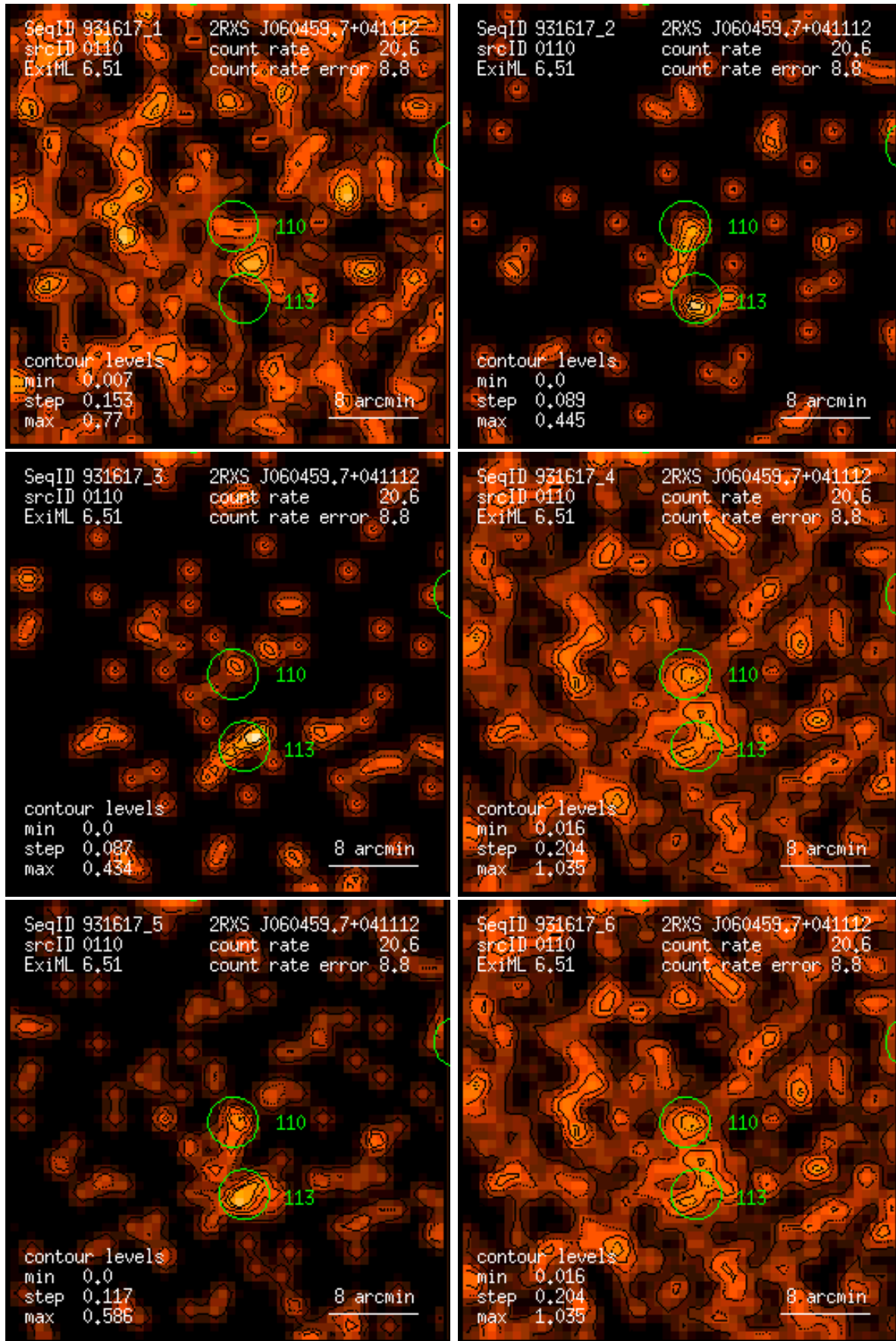
Figure 110: RASS 931617: detection 0110: band rate images, Gaussian filter: (1) PSPC channels 11 – 41, (2) 52 – 90, (3) 91 – 201, (4) 11 – 235, (5) 52 – 201, (6) 11 – 201. Broad band rates in counts/ks. Band rate contour levels in counts/ks/arcmin 2 .
