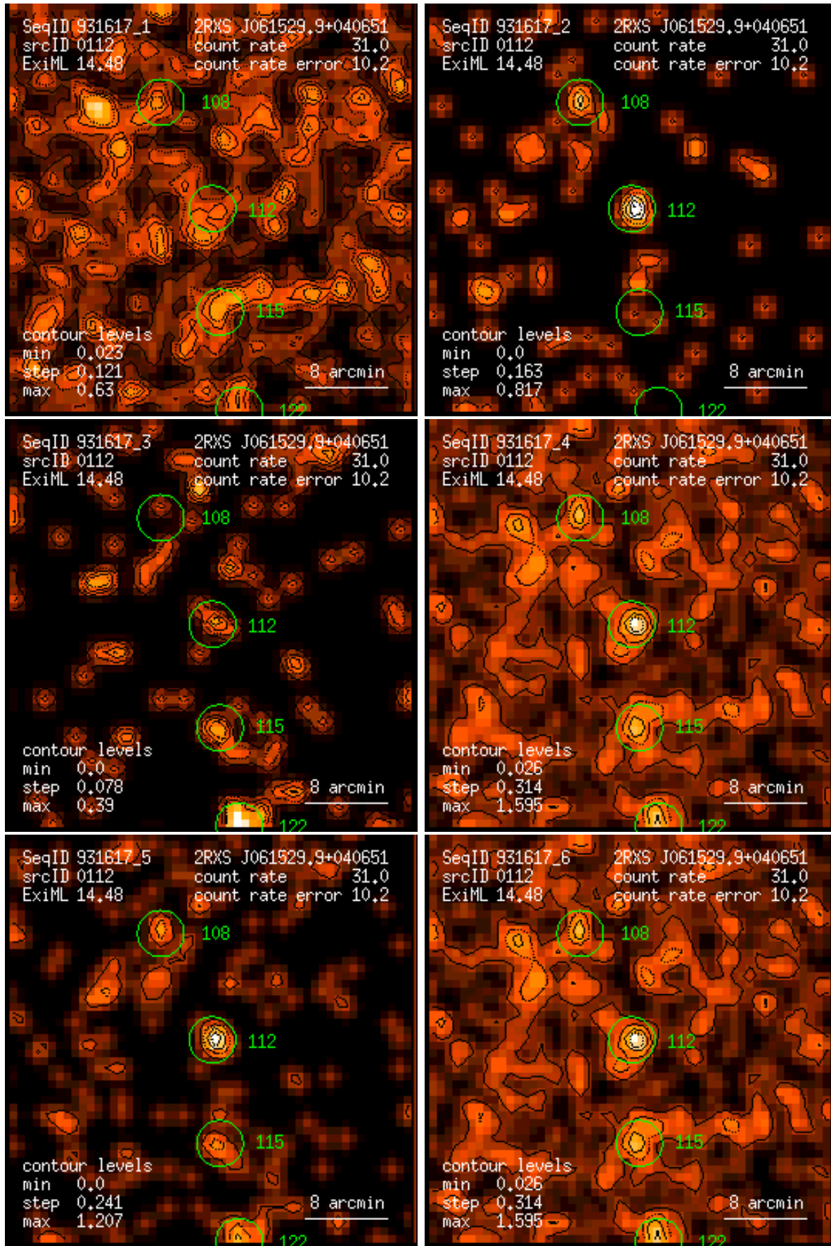
Figure 112: RASS 931617: detection 0112: band rate images, Gaussian filter: (1) PSPC channels 11 – 41, (2) 52 – 90, (3) 91 – 201, (4) 11 – 235, (5) 52 – 201, (6) 11 – 201. Broad band rates in counts/ks. Band rate contour levels in counts/ks/arcmin 2 .
