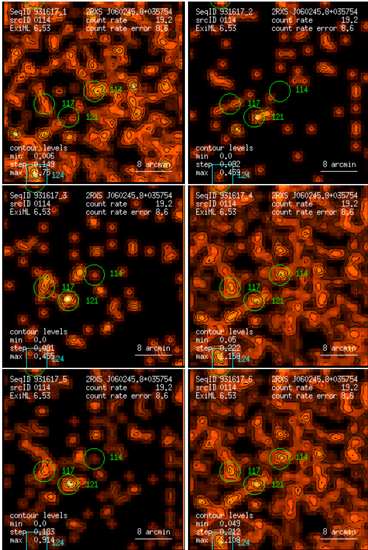
Figure 114: RASS 931617: detection 0114: band rate images, Gaussian filter: (1) PSPC channels 11 – 41, (2) 52 – 90, (3) 91 – 201, (4) 11 – 235, (5) 52 – 201, (6) 11 – 201. Broad band rates in counts/ks. Band rate contour levels in counts/ks/arcmin 2 .
