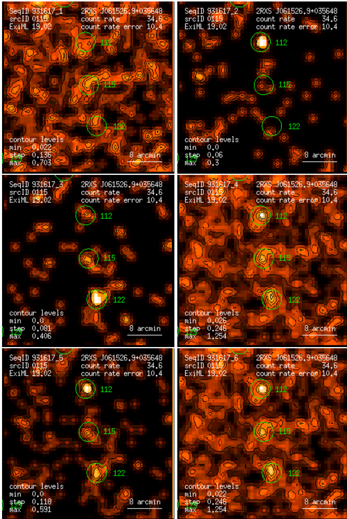
Figure 115: RASS 931617: detection 0115: band rate images, Gaussian filter: (1) PSPC channels 11 – 41, (2) 52 – 90, (3) 91 – 201, (4) 11 – 235, (5) 52 – 201, (6) 11 – 201. Broad band rates in counts/ks. Band rate contour levels in counts/ks/arcmin 2 .
