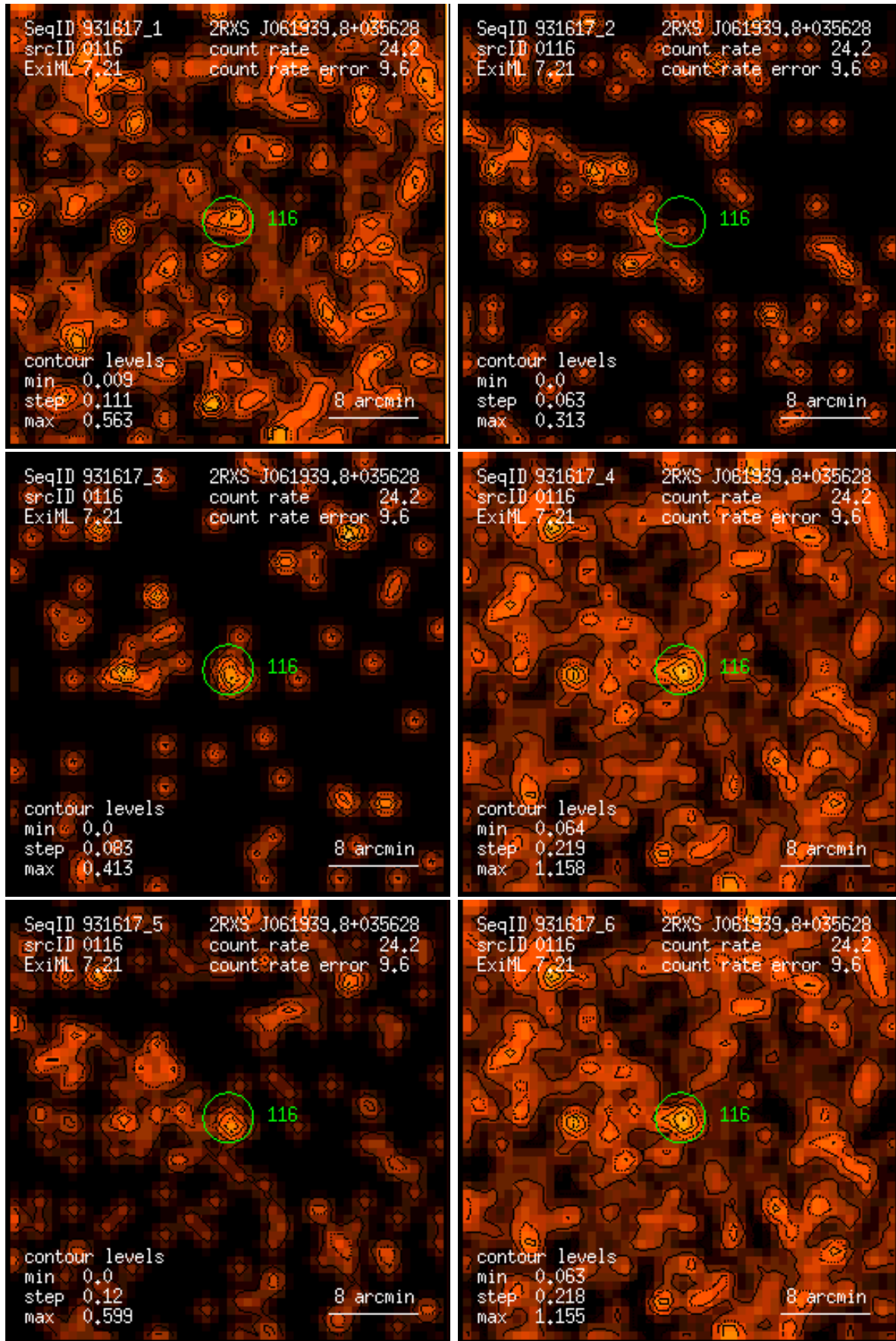
Figure 116: RASS 931617: detection 0116: band rate images, Gaussian filter: (1) PSPC channels 11 – 41, (2) 52 – 90, (3) 91 – 201, (4) 11 – 235, (5) 52 – 201, (6) 11 – 201. Broad band rates in counts/ks. Band rate contour levels in counts/ks/arcmin 2 .
