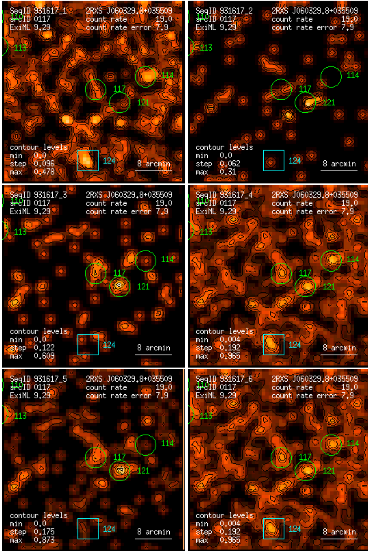
Figure 117: RASS 931617: detection 0117: band rate images, Gaussian filter: (1) PSPC channels 11 – 41, (2) 52 – 90, (3) 91 – 201, (4) 11 – 235, (5) 52 – 201, (6) 11 – 201. Broad band rates in counts/ks. Band rate contour levels in counts/ks/arcmin 2 .
