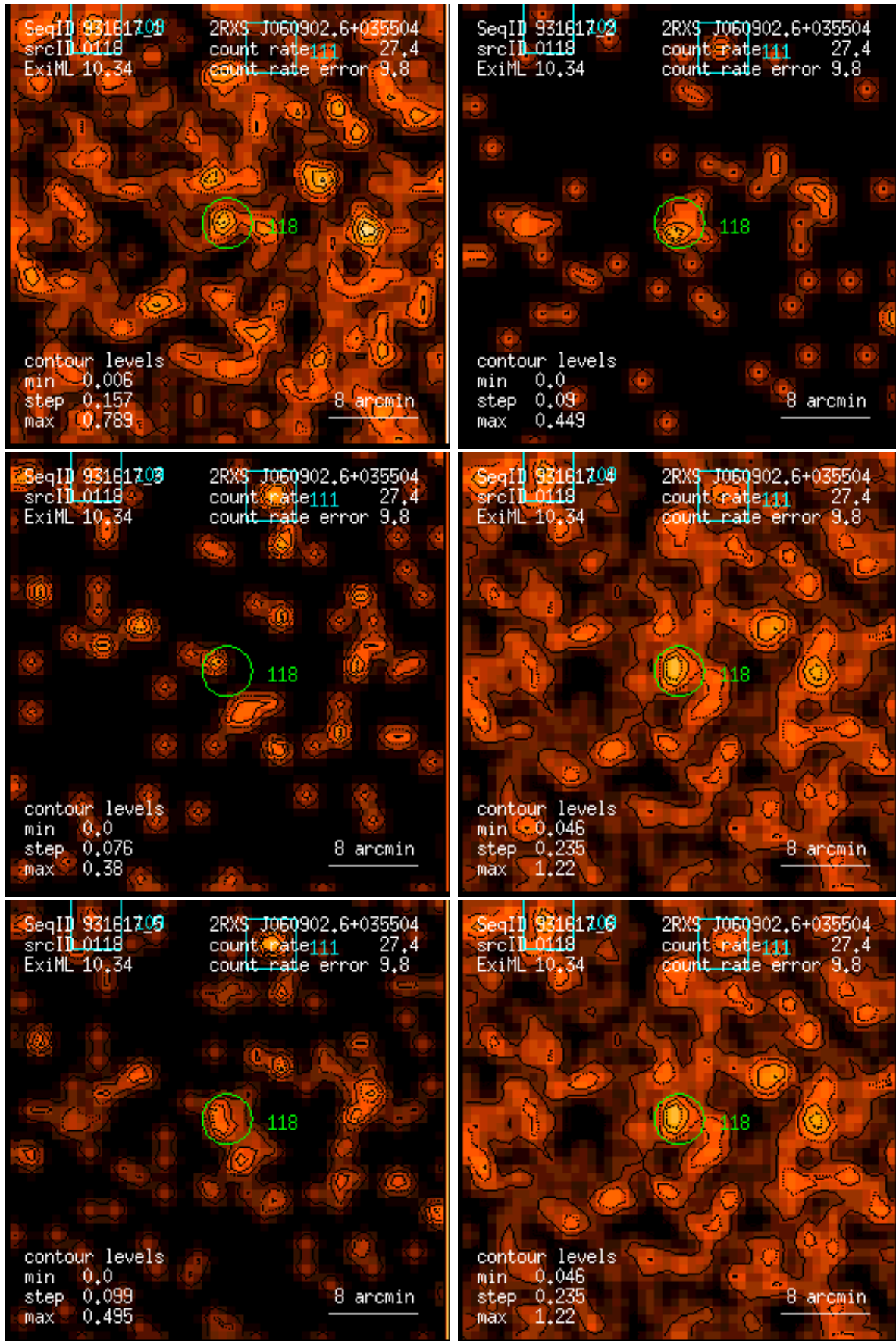
Figure 118: RASS 931617: detection 0118: band rate images, Gaussian filter: (1) PSPC channels 11 – 41, (2) 52 – 90, (3) 91 – 201, (4) 11 – 235, (5) 52 – 201, (6) 11 – 201. Broad band rates in counts/ks. Band rate contour levels in counts/ks/arcmin 2 .
