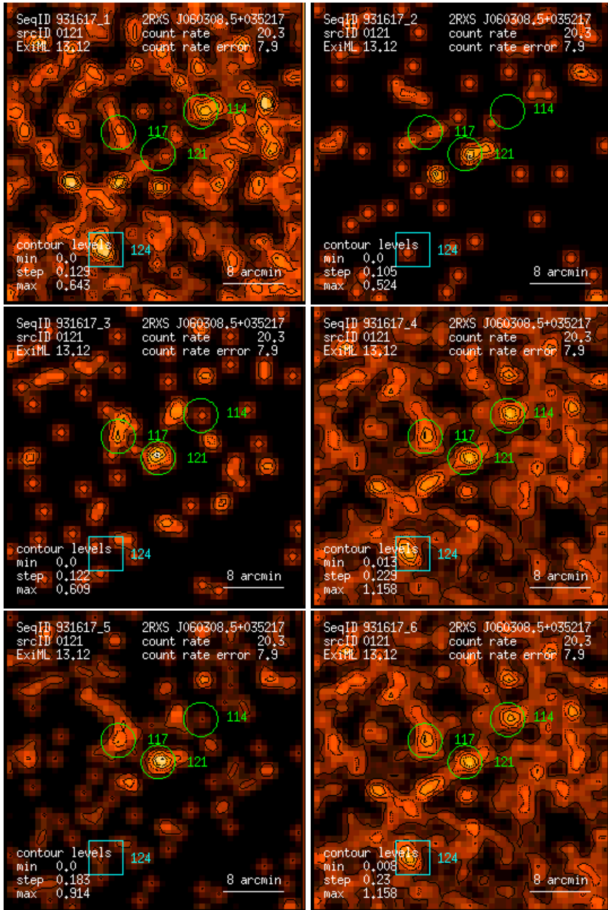
Figure 121: RASS 931617: detection 0121: band rate images, Gaussian filter: (1) PSPC channels 11 – 41, (2) 52 – 90, (3) 91 – 201, (4) 11 – 235, (5) 52 – 201, (6) 11 – 201. Broad band rates in counts/ks. Band rate contour levels in counts/ks/arcmin 2 .
