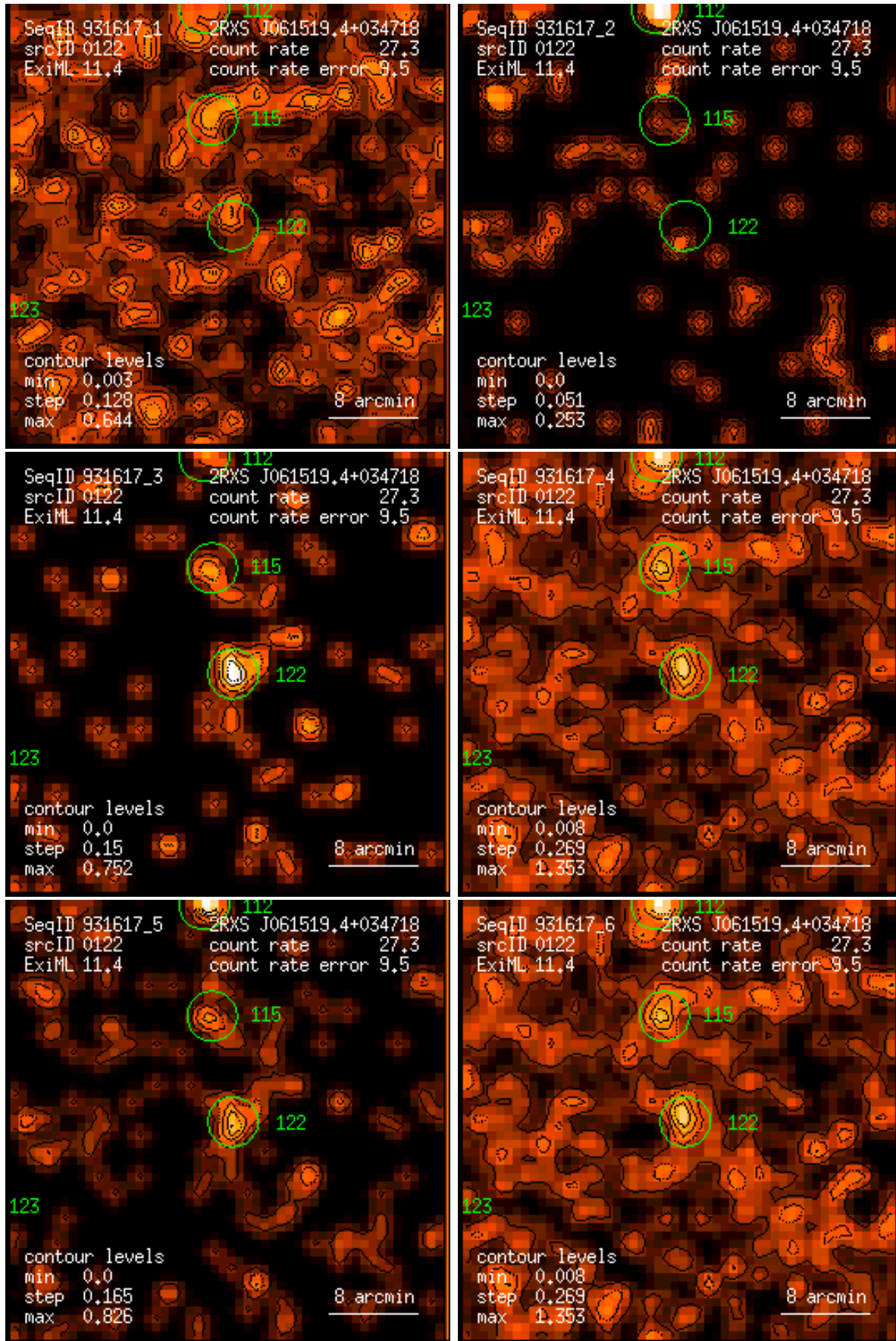
Figure 122: RASS 931617: detection 0122: band rate images, Gaussian filter: (1) PSPC channels 11 – 41, (2) 52 – 90, (3) 91 – 201, (4) 11 – 235, (5) 52 – 201, (6) 11 – 201. Broad band rates in counts/ks. Band rate contour levels in counts/ks/arcmin 2 .
