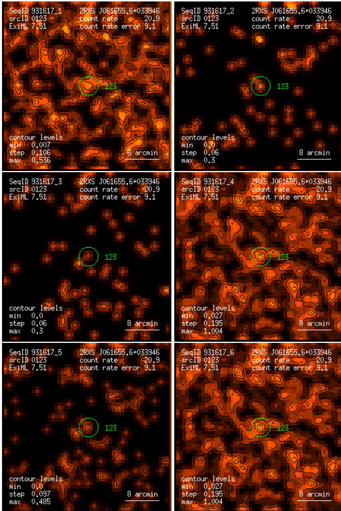
Figure 123: RASS 931617: detection 0123: band rate images, Gaussian filter: (1) PSPC channels 11 – 41, (2) 52 – 90, (3) 91 – 201, (4) 11 – 235, (5) 52 – 201, (6) 11 – 201. Broad band rates in counts/ks. Band rate contour levels in counts/ks/arcmin 2 .
