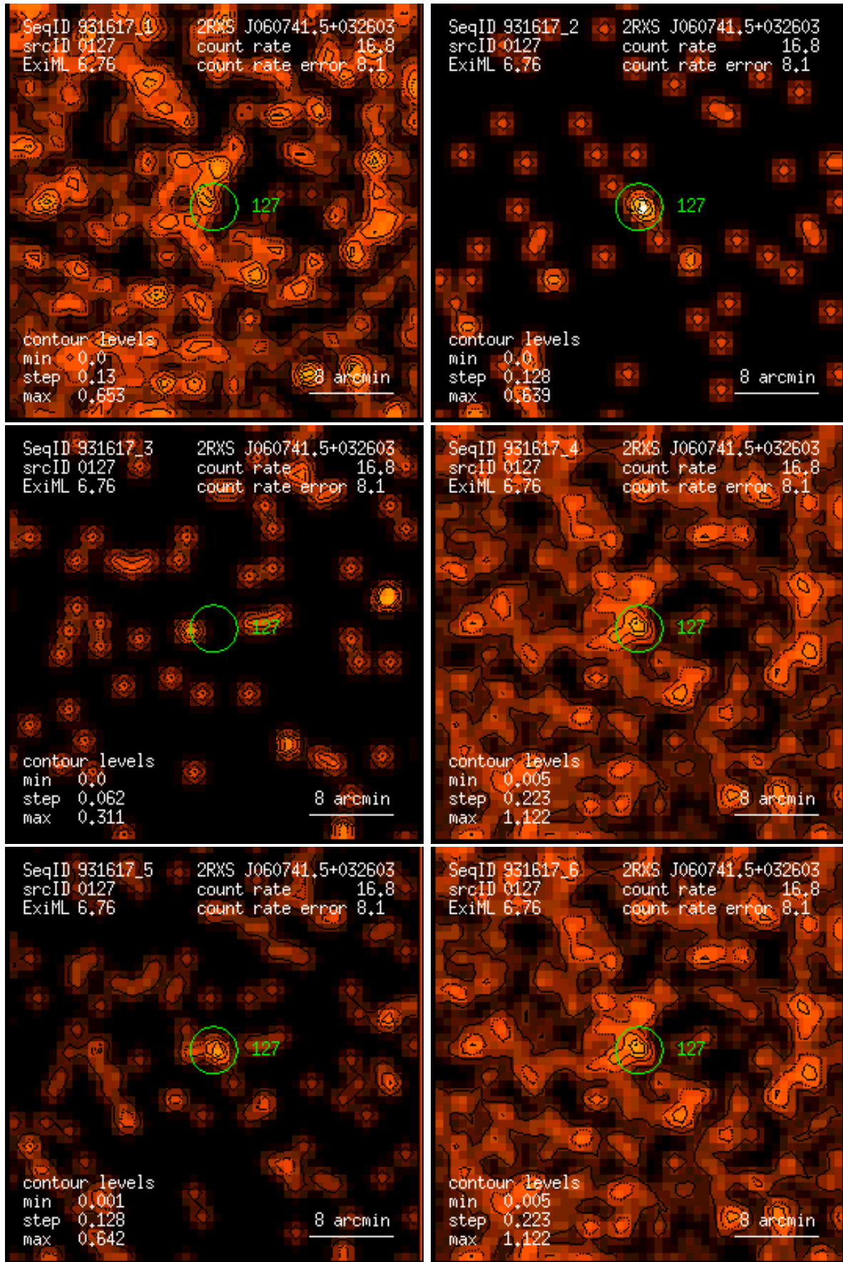
Figure 127: RASS 931617: detection 0127: band rate images, Gaussian filter: (1) PSPC channels 11 – 41, (2) 52 – 90, (3) 91 – 201, (4) 11 – 235, (5) 52 – 201, (6) 11 – 201. Broad band rates in counts/ks. Band rate contour levels in counts/ks/arcmin 2 .
