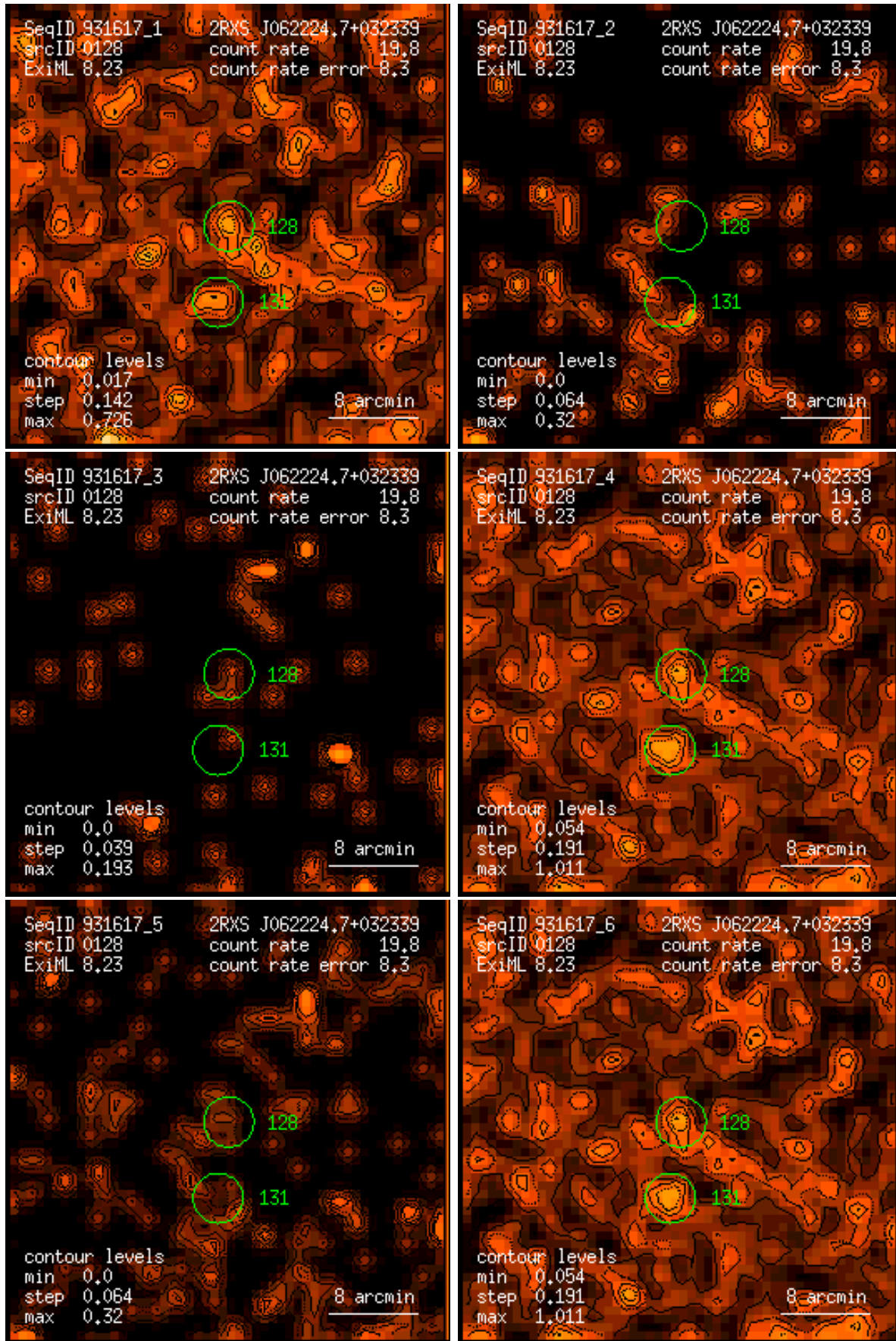
Figure 128: RASS 931617: detection 0128: band rate images, Gaussian filter: (1) PSPC channels 11 – 41, (2) 52 – 90, (3) 91 – 201, (4) 11 – 235, (5) 52 – 201, (6) 11 – 201. Broad band rates in counts/ks. Band rate contour levels in counts/ks/arcmin 2 .
