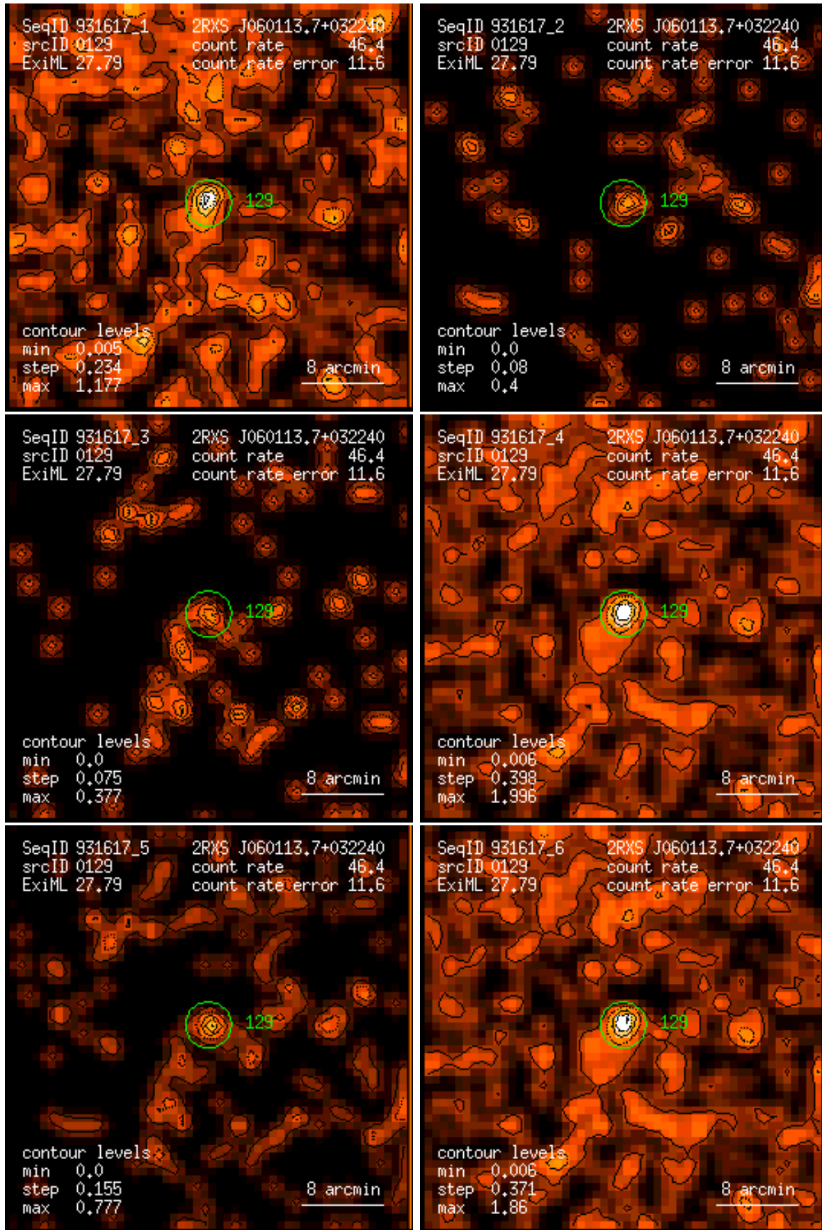
Figure 129: RASS 931617: detection 0129: band rate images, Gaussian filter: (1) PSPC channels 11 – 41, (2) 52 – 90, (3) 91 – 201, (4) 11 – 235, (5) 52 – 201, (6) 11 – 201. Broad band rates in counts/ks. Band rate contour levels in counts/ks/arcmin 2 .
