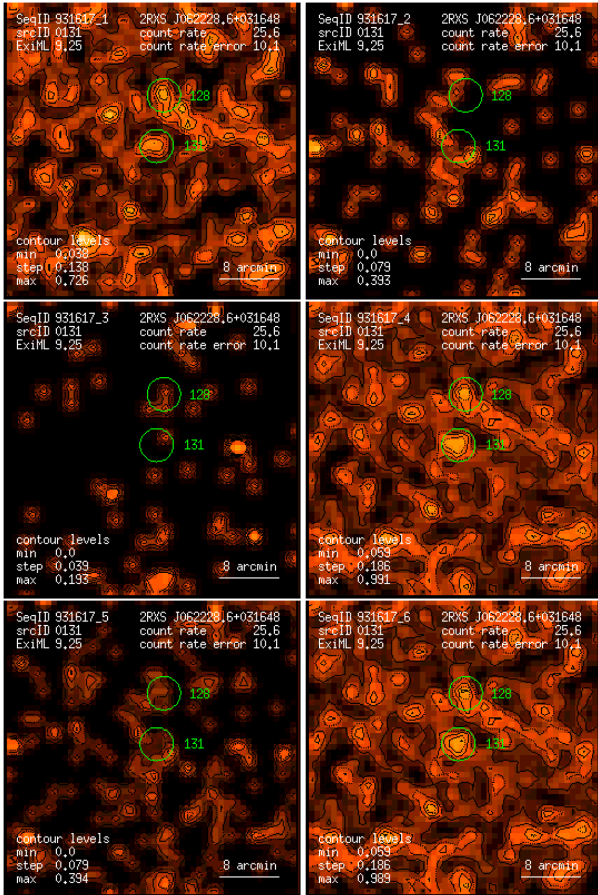
Figure 131: RASS 931617: detection 0131: band rate images, Gaussian filter: (1) PSPC channels 11 – 41, (2) 52 – 90, (3) 91 – 201, (4) 11 – 235, (5) 52 – 201, (6) 11 – 201. Broad band rates in counts/ks. Band rate contour levels in counts/ks/arcmin 2 .
