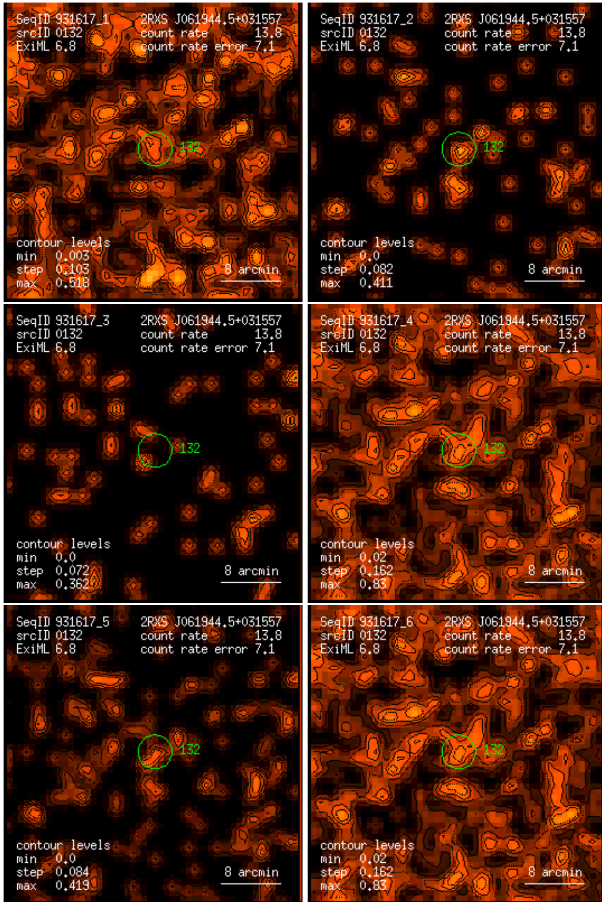
Figure 132: RASS 931617: detection 0132: band rate images, Gaussian filter: (1) PSPC channels 11 – 41, (2) 52 – 90, (3) 91 – 201, (4) 11 – 235, (5) 52 – 201, (6) 11 – 201. Broad band rates in counts/ks. Band rate contour levels in counts/ks/arcmin 2 .
