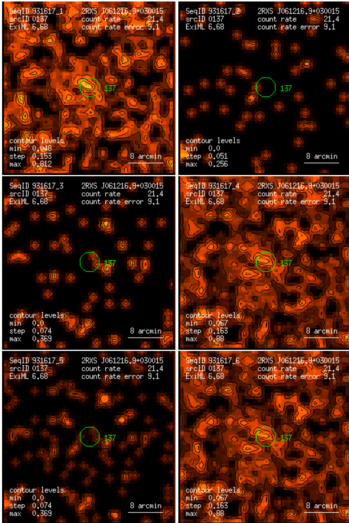
Figure 137: RASS 931617: detection 0137: band rate images, Gaussian filter: (1) PSPC channels 11 – 41, (2) 52 – 90, (3) 91 – 201, (4) 11 – 235, (5) 52 – 201, (6) 11 – 201. Broad band rates in counts/ks. Band rate contour levels in counts/ks/arcmin 2 .
