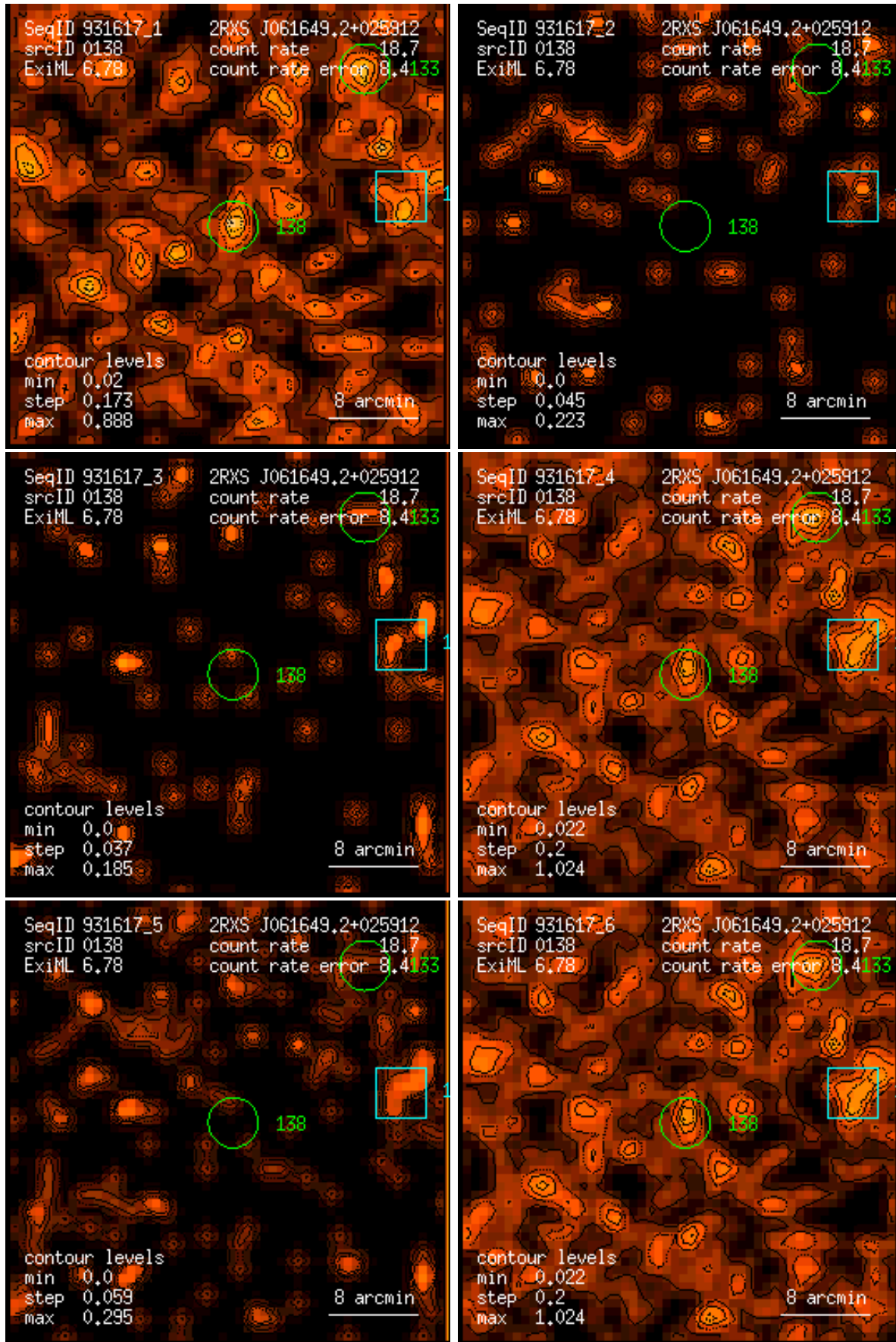
Figure 138: RASS 931617: detection 0138: band rate images, Gaussian filter: (1) PSPC channels 11 – 41, (2) 52 – 90, (3) 91 – 201, (4) 11 – 235, (5) 52 – 201, (6) 11 – 201. Broad band rates in counts/ks. Band rate contour levels in counts/ks/arcmin 2 .
