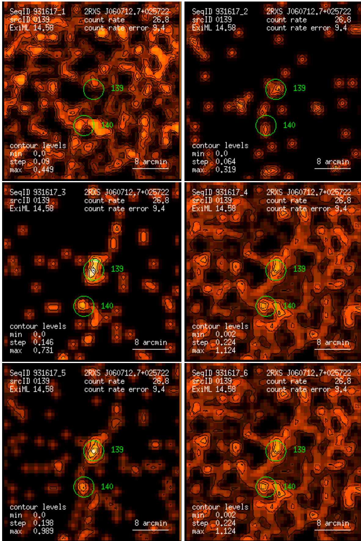
Figure 139: RASS 931617: detection 0139: band rate images, Gaussian filter: (1) PSPC channels 11 – 41, (2) 52 – 90, (3) 91 – 201, (4) 11 – 235, (5) 52 – 201, (6) 11 – 201. Broad band rates in counts/ks. Band rate contour levels in counts/ks/arcmin 2 .
