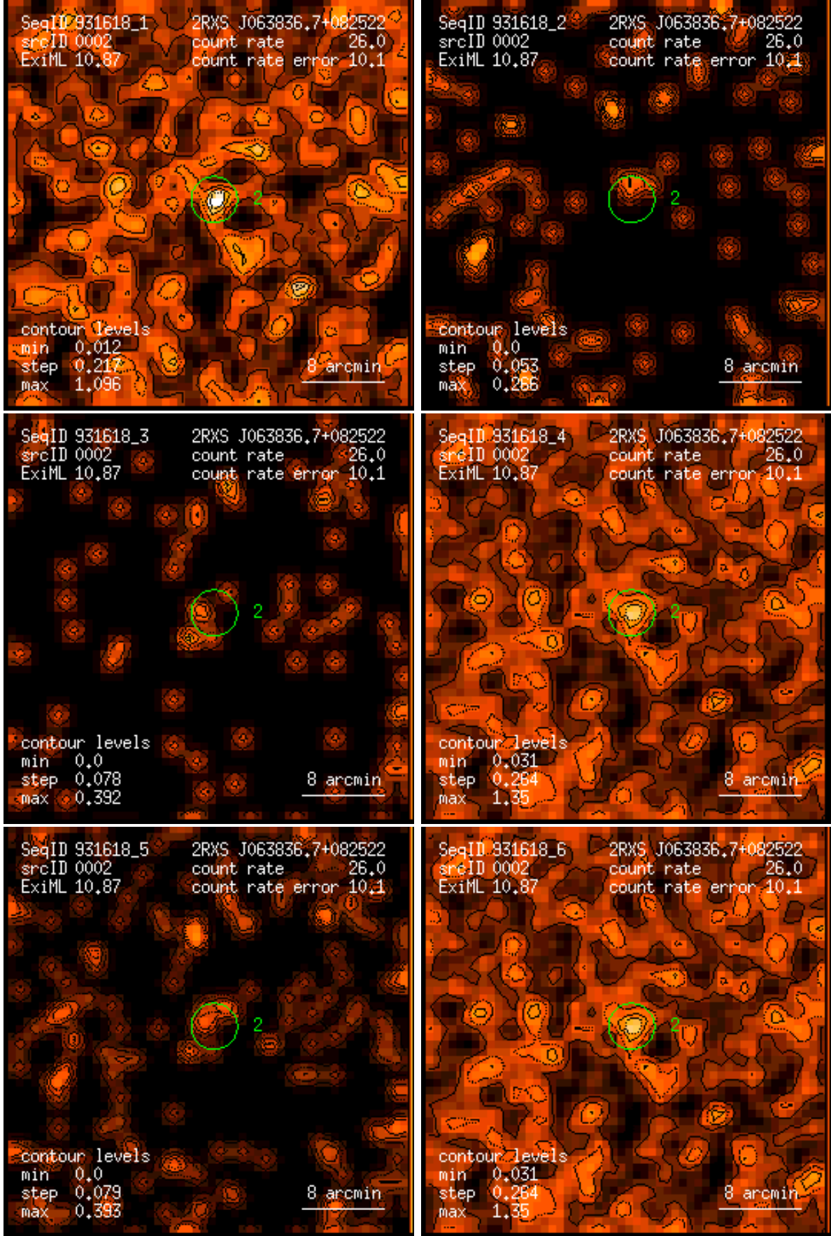
Figure 2: RASS 931618: detection 0002: band rate images, Gaussian filter: (1) PSPC channels 11 – 41, (2) 52 – 90, (3) 91 – 201, (4) 11 – 235, (5) 52 – 201, (6) 11 – 201. Broad band rates in counts/ks. Band rate contour levels in counts/ks/arcmin 2 .
