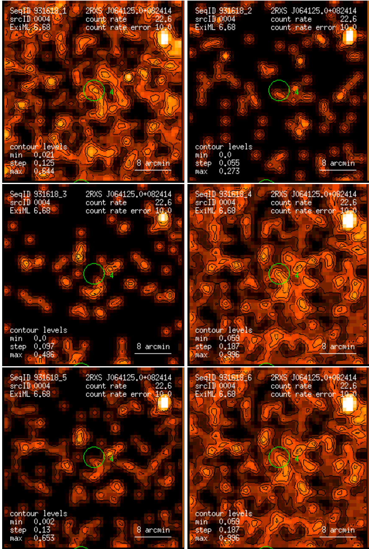
Figure 4: RASS 931618: detection 0004: band rate images, Gaussian filter: (1) PSPC channels 11 – 41, (2) 52 – 90, (3) 91 – 201, (4) 11 – 235, (5) 52 – 201, (6) 11 – 201. Broad band rates in counts/ks. Band rate contour levels in counts/ks/arcmin 2 .
