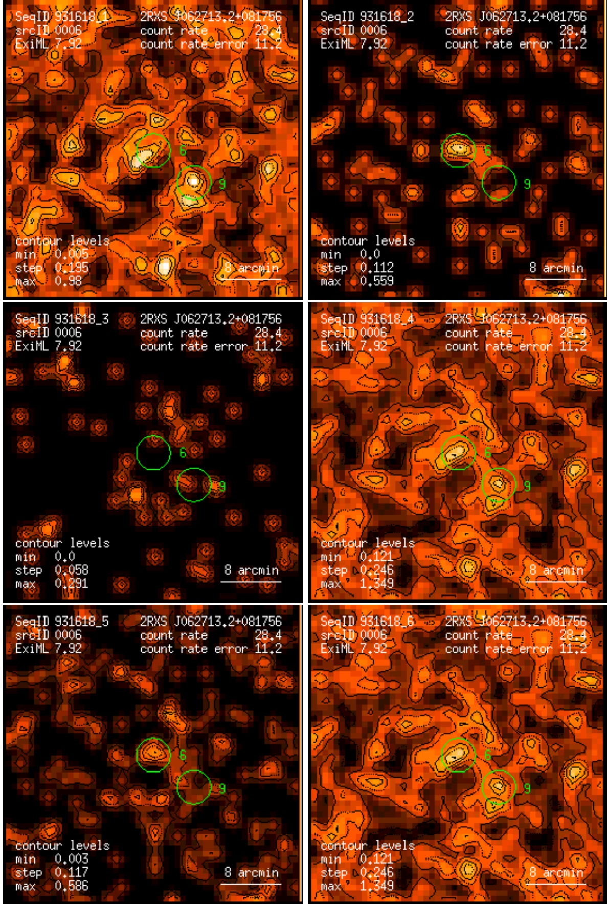
Figure 6: RASS 931618: detection 0006: band rate images, Gaussian filter: (1) PSPC channels 11 – 41, (2) 52 – 90, (3) 91 – 201, (4) 11 – 235, (5) 52 – 201, (6) 11 – 201. Broad band rates in counts/ks. Band rate contour levels in counts/ks/arcmin 2 .
