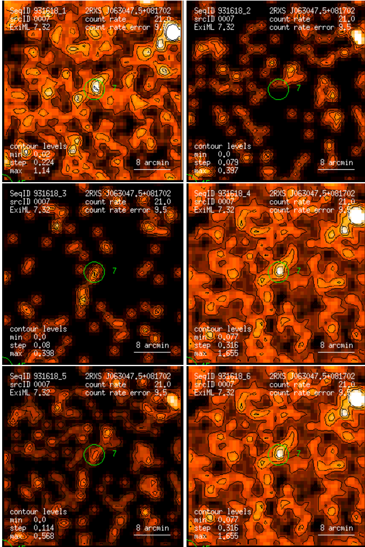
Figure 7: RASS 931618: detection 0007: band rate images, Gaussian filter: (1) PSPC channels 11 – 41, (2) 52 – 90, (3) 91 – 201, (4) 11 – 235, (5) 52 – 201, (6) 11 – 201. Broad band rates in counts/ks. Band rate contour levels in counts/ks/arcmin 2 .
