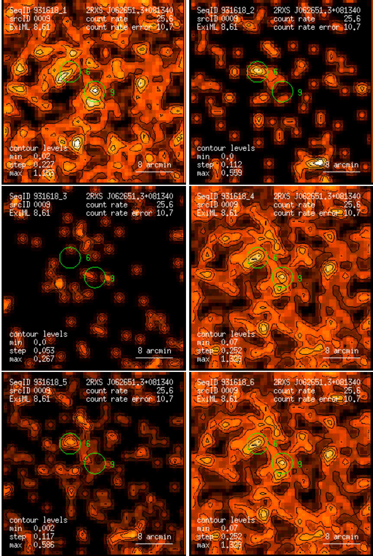
Figure 9: RASS 931618: detection 0009: band rate images, Gaussian filter: (1) PSPC channels 11 – 41, (2) 52 – 90, (3) 91 – 201, (4) 11 – 235, (5) 52 – 201, (6) 11 – 201. Broad band rates in counts/ks. Band rate contour levels in counts/ks/arcmin 2 .
