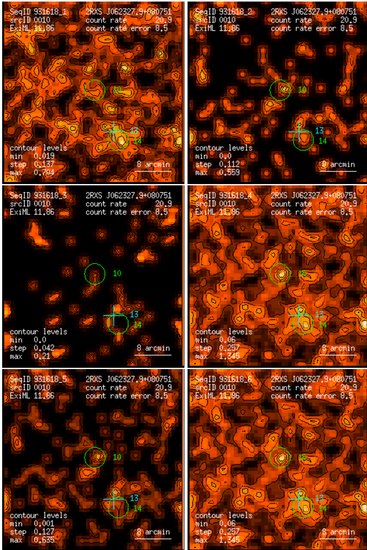
Figure 10: RASS 931618: detection 0010: band rate images, Gaussian filter: (1) PSPC channels 11 – 41, (2) 52 – 90, (3) 91 – 201, (4) 11 – 235, (5) 52 – 201, (6) 11 – 201. Broad band rates in counts/ks. Band rate contour levels in counts/ks/arcmin 2 .
