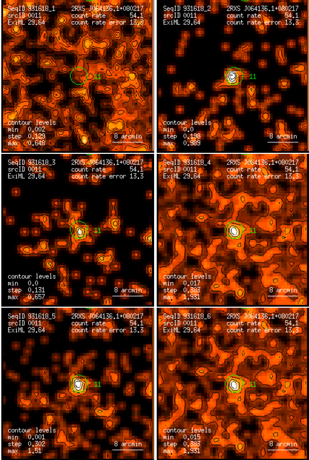
Figure 11: RASS 931618: detection 0011: band rate images, Gaussian filter: (1) PSPC channels 11 – 41, (2) 52 – 90, (3) 91 – 201, (4) 11 – 235, (5) 52 – 201, (6) 11 – 201. Broad band rates in counts/ks. Band rate contour levels in counts/ks/arcmin 2 .
