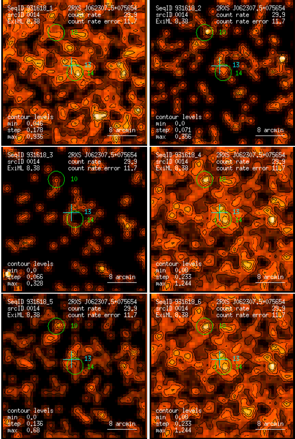
Figure 14: RASS 931618: detection 0014: band rate images, Gaussian filter: (1) PSPC channels 11 – 41, (2) 52 – 90, (3) 91 – 201, (4) 11 – 235, (5) 52 – 201, (6) 11 – 201. Broad band rates in counts/ks. Band rate contour levels in counts/ks/arcmin 2 .
