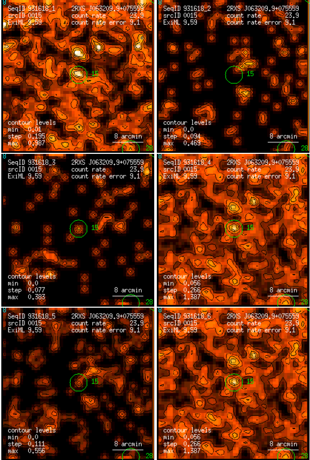
Figure 15: RASS 931618: detection 0015: band rate images, Gaussian filter: (1) PSPC channels 11 – 41, (2) 52 – 90, (3) 91 – 201, (4) 11 – 235, (5) 52 – 201, (6) 11 – 201. Broad band rates in counts/ks. Band rate contour levels in counts/ks/arcmin 2 .
