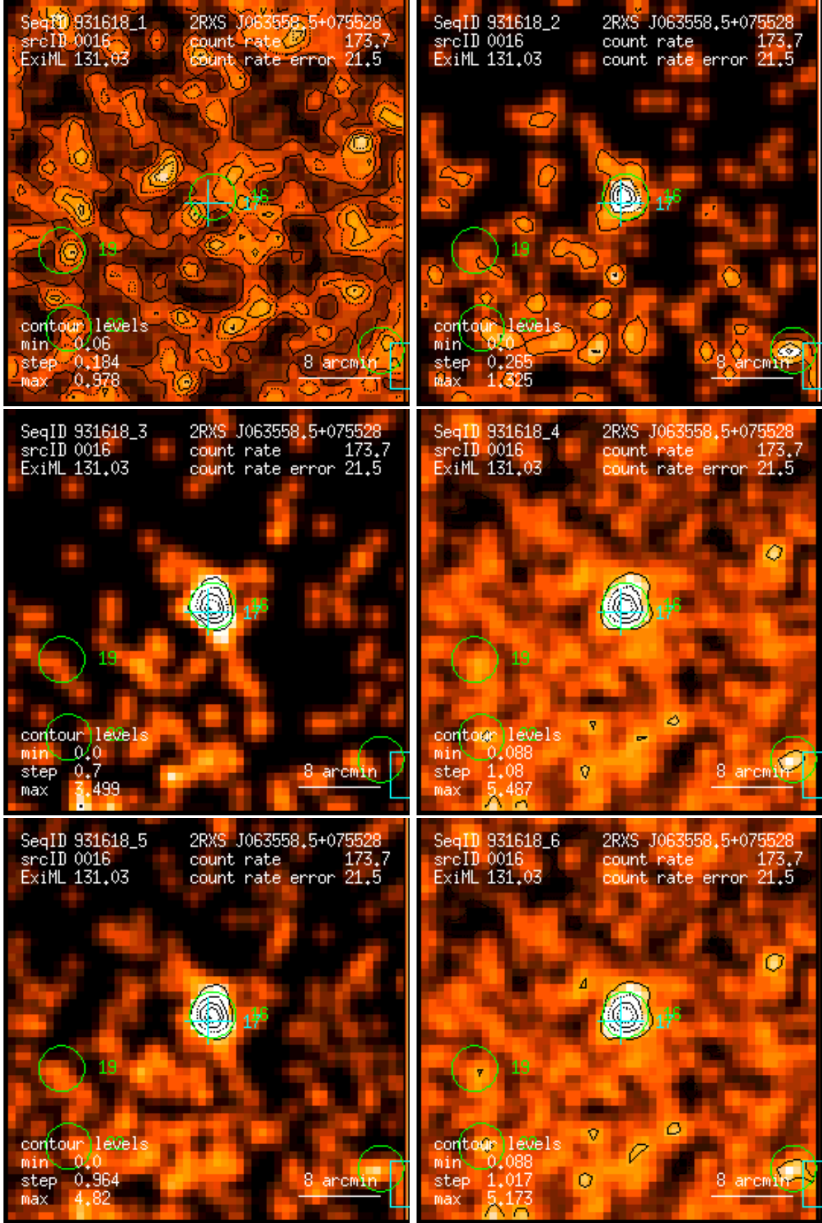
Figure 16: RASS 931618: detection 0016: band rate images, Gaussian filter: (1) PSPC channels 11 – 41, (2) 52 – 90, (3) 91 – 201, (4) 11 – 235, (5) 52 – 201, (6) 11 – 201. Broad band rates in counts/ks. Band rate contour levels in counts/ks/arcmin 2 .
