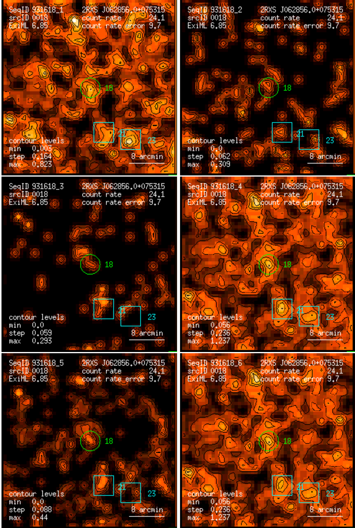
Figure 18: RASS 931618: detection 0018: band rate images, Gaussian filter: (1) PSPC channels 11 – 41, (2) 52 – 90, (3) 91 – 201, (4) 11 – 235, (5) 52 – 201, (6) 11 – 201. Broad band rates in counts/ks. Band rate contour levels in counts/ks/arcmin 2 .
