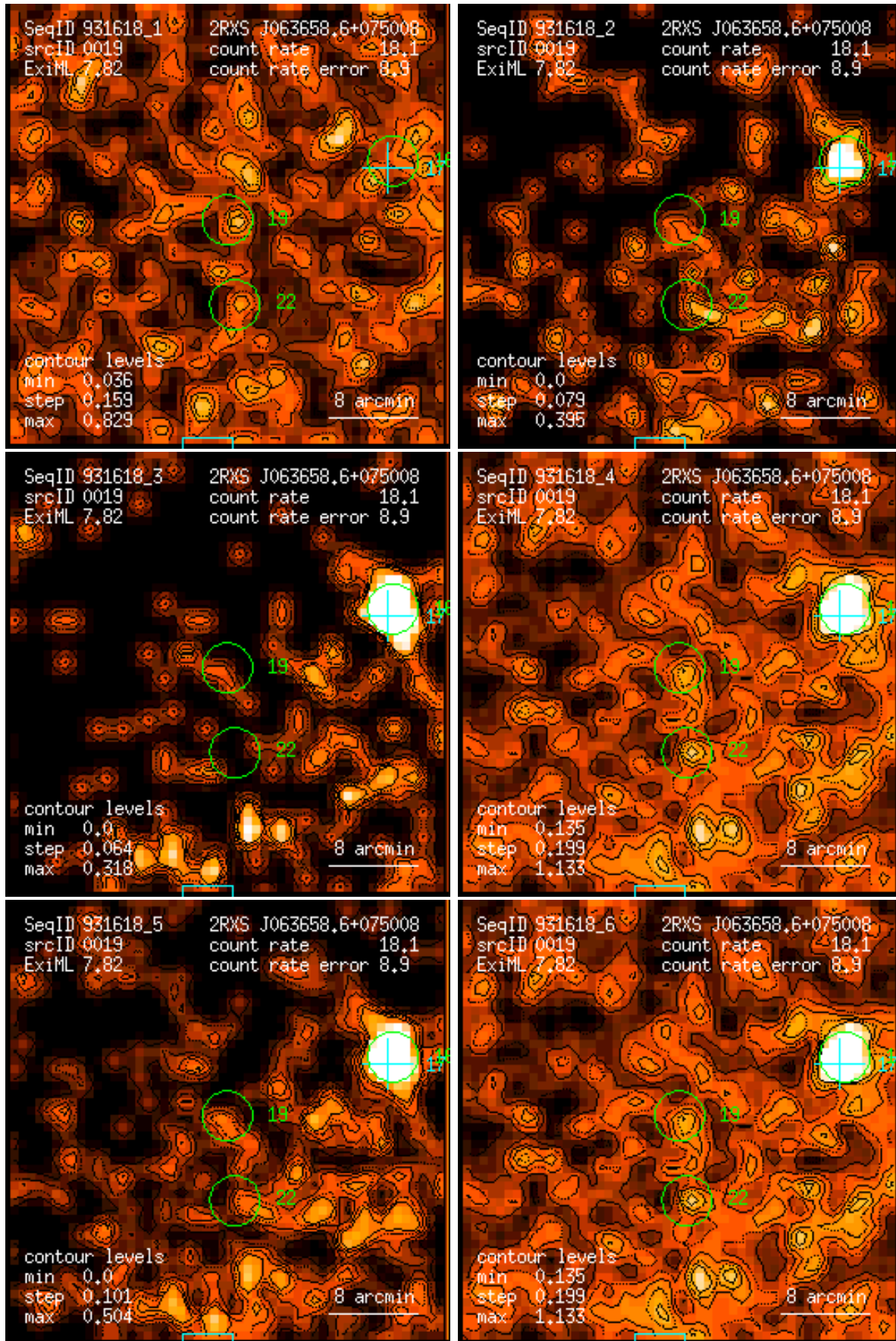
Figure 19: RASS 931618: detection 0019: band rate images, Gaussian filter: (1) PSPC channels 11 – 41, (2) 52 – 90, (3) 91 – 201, (4) 11 – 235, (5) 52 – 201, (6) 11 – 201. Broad band rates in counts/ks. Band rate contour levels in counts/ks/arcmin 2 .
