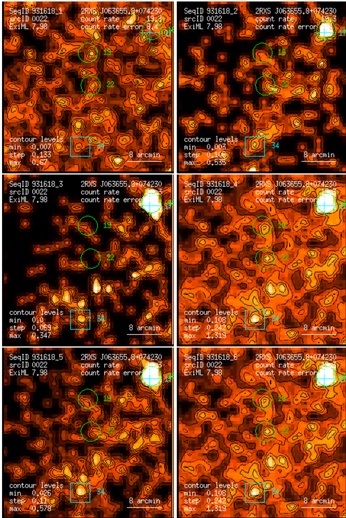
Figure 22: RASS 931618: detection 0022: band rate images, Gaussian filter: (1) PSPC channels 11 – 41, (2) 52 – 90, (3) 91 – 201, (4) 11 – 235, (5) 52 – 201, (6) 11 – 201. Broad band rates in counts/ks. Band rate contour levels in counts/ks/arcmin 2 .
