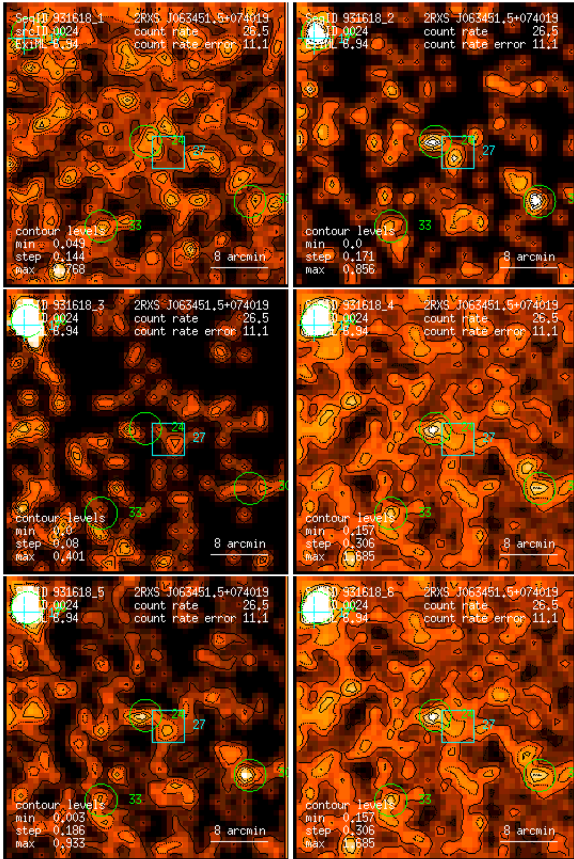
Figure 24: RASS 931618: detection 0024: band rate images, Gaussian filter: (1) PSPC channels 11 – 41, (2) 52 – 90, (3) 91 – 201, (4) 11 – 235, (5) 52 – 201, (6) 11 – 201. Broad band rates in counts/ks. Band rate contour levels in counts/ks/arcmin 2 .
