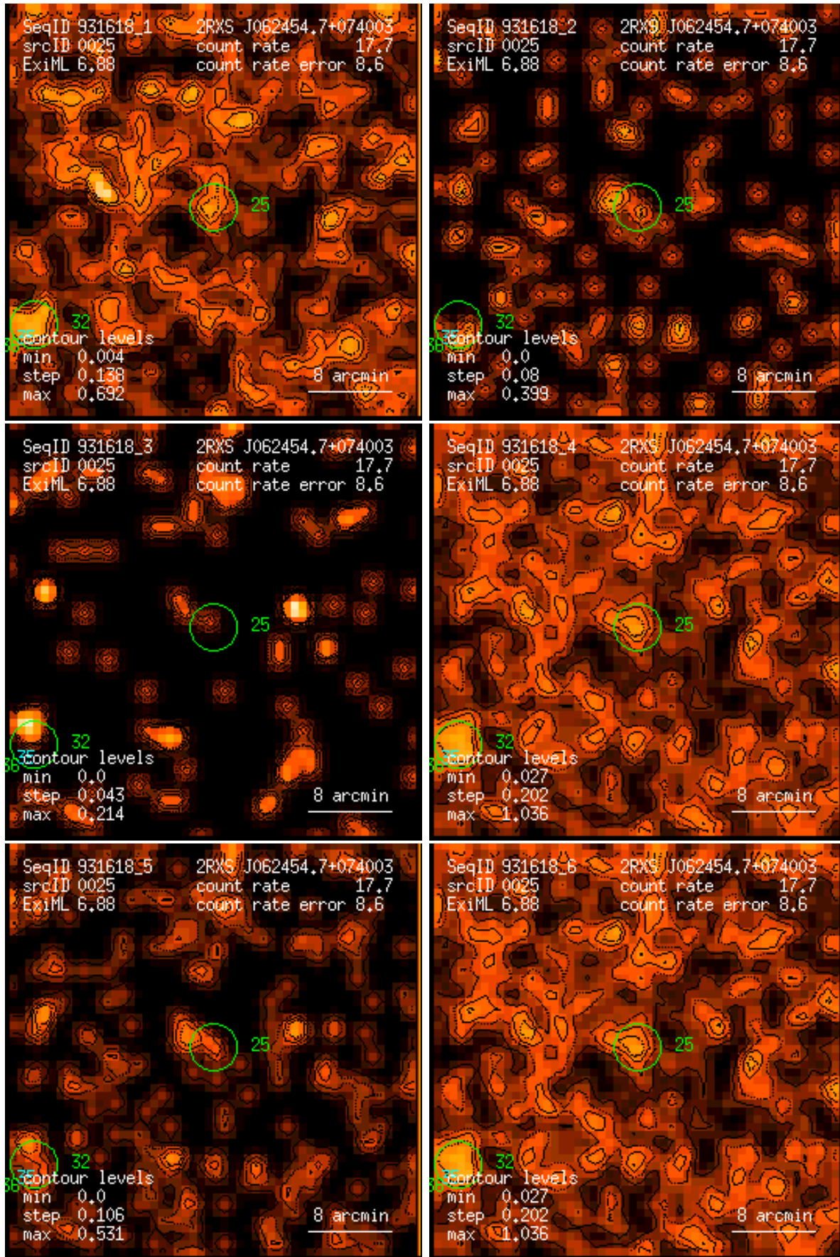
Figure 25: RASS 931618: detection 0025: band rate images, Gaussian filter: (1) PSPC channels 11 – 41, (2) 52 – 90, (3) 91 – 201, (4) 11 – 235, (5) 52 – 201, (6) 11 – 201. Broad band rates in counts/ks. Band rate contour levels in counts/ks/arcmin 2 .
