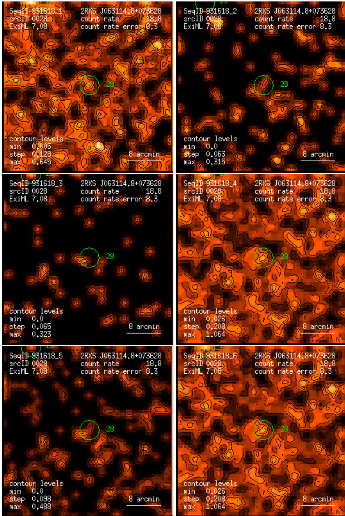
Figure 28: RASS 931618: detection 0028: band rate images, Gaussian filter: (1) PSPC channels 11 – 41, (2) 52 – 90, (3) 91 – 201, (4) 11 – 235, (5) 52 – 201, (6) 11 – 201. Broad band rates in counts/ks. Band rate contour levels in counts/ks/arcmin 2 .
