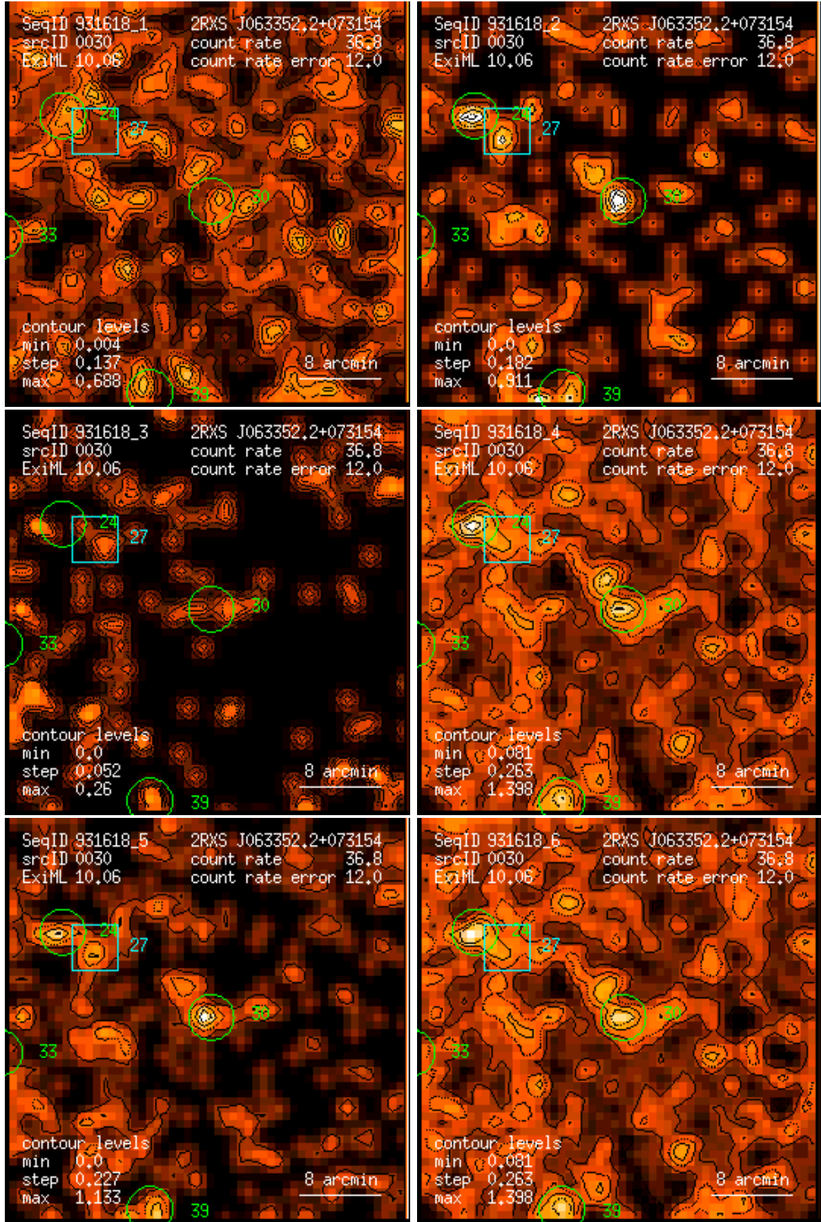
Figure 30: RASS 931618: detection 0030: band rate images, Gaussian filter: (1) PSPC channels 11 – 41, (2) 52 – 90, (3) 91 – 201, (4) 11 – 235, (5) 52 – 201, (6) 11 – 201. Broad band rates in counts/ks. Band rate contour levels in counts/ks/arcmin 2 .
