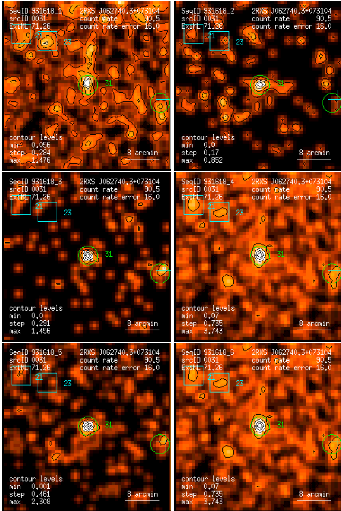
Figure 31: RASS 931618: detection 0031: band rate images, Gaussian filter: (1) PSPC channels 11 – 41, (2) 52 – 90, (3) 91 – 201, (4) 11 – 235, (5) 52 – 201, (6) 11 – 201. Broad band rates in counts/ks. Band rate contour levels in counts/ks/arcmin 2 .
