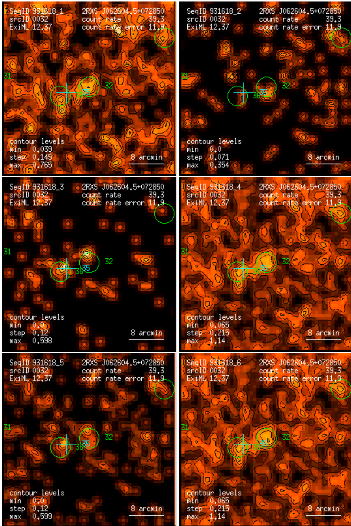
Figure 32: RASS 931618: detection 0032: band rate images, Gaussian filter: (1) PSPC channels 11 – 41, (2) 52 – 90, (3) 91 – 201, (4) 11 – 235, (5) 52 – 201, (6) 11 – 201. Broad band rates in counts/ks. Band rate contour levels in counts/ks/arcmin 2 .
