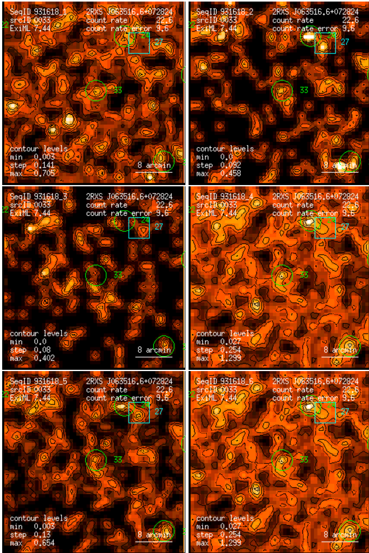
Figure 33: RASS 931618: detection 0033: band rate images, Gaussian filter: (1) PSPC channels 11 – 41, (2) 52 – 90, (3) 91 – 201, (4) 11 – 235, (5) 52 – 201, (6) 11 – 201. Broad band rates in counts/ks. Band rate contour levels in counts/ks/arcmin 2 .
