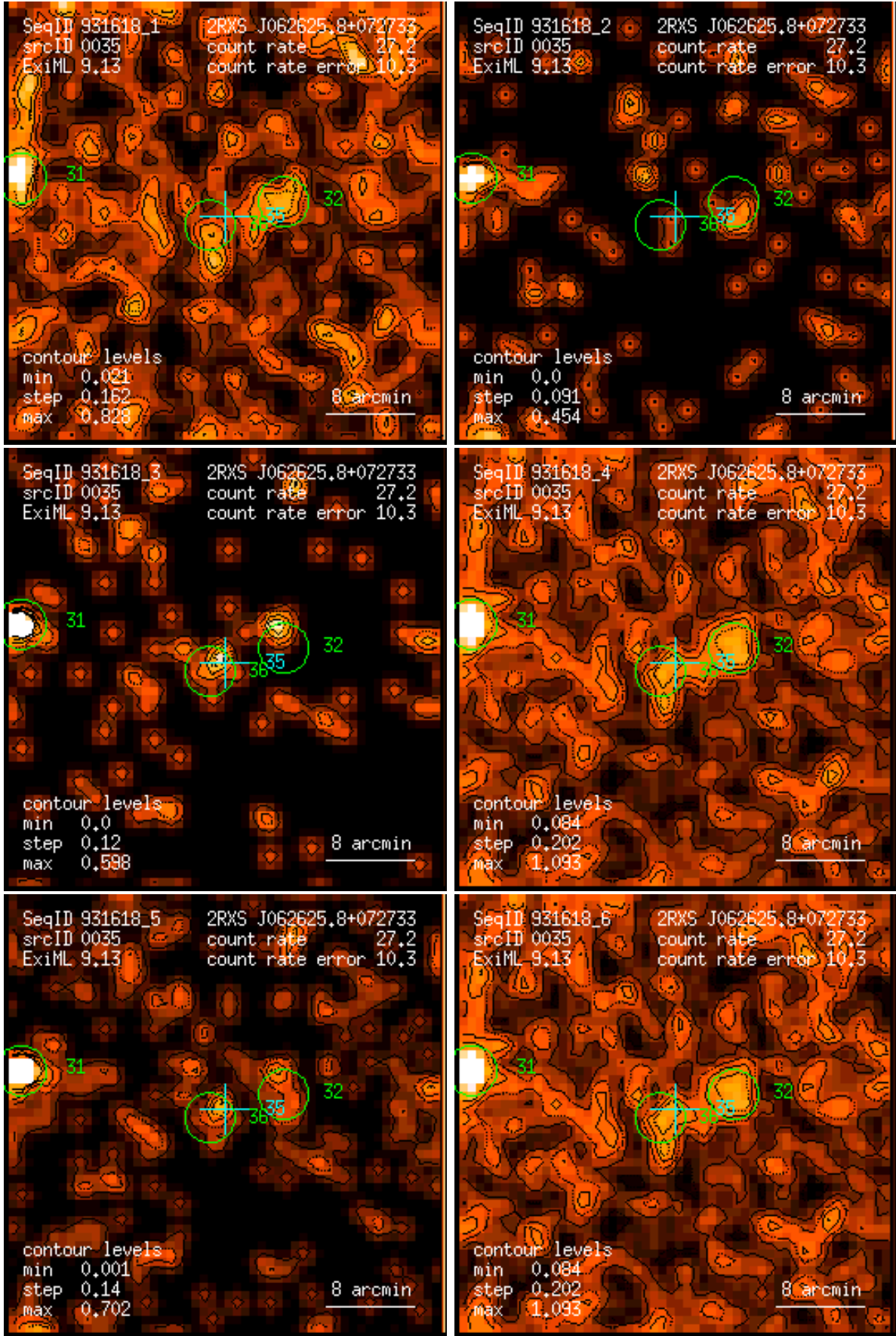
Figure 35: RASS 931618: detection 0035: band rate images, Gaussian filter: (1) PSPC channels 11 – 41, (2) 52 – 90, (3) 91 – 201, (4) 11 – 235, (5) 52 – 201, (6) 11 – 201. Broad band rates in counts/ks. Band rate contour levels in counts/ks/arcmin 2 .
