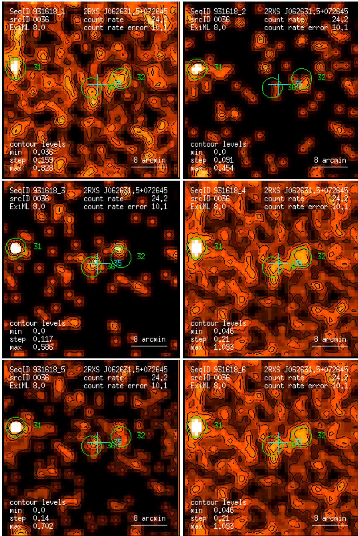
Figure 36: RASS 931618: detection 0036: band rate images, Gaussian filter: (1) PSPC channels 11 – 41, (2) 52 – 90, (3) 91 – 201, (4) 11 – 235, (5) 52 – 201, (6) 11 – 201. Broad band rates in counts/ks. Band rate contour levels in counts/ks/arcmin 2 .
