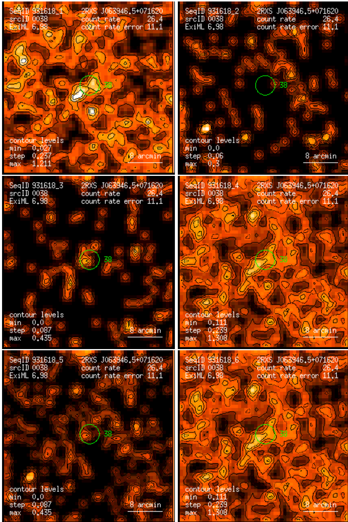
Figure 38: RASS 931618: detection 0038: band rate images, Gaussian filter: (1) PSPC channels 11 – 41, (2) 52 – 90, (3) 91 – 201, (4) 11 – 235, (5) 52 – 201, (6) 11 – 201. Broad band rates in counts/ks. Band rate contour levels in counts/ks/arcmin 2 .
