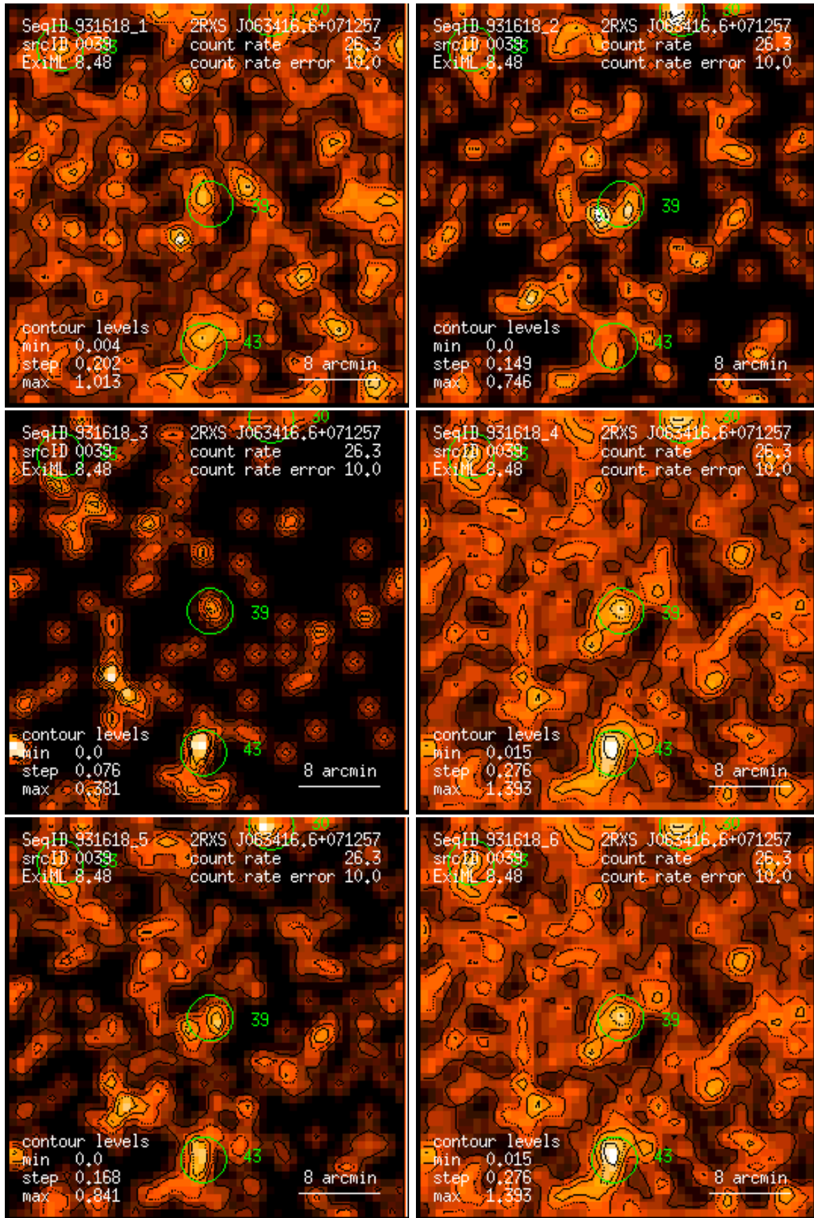
Figure 39: RASS 931618: detection 0039: band rate images, Gaussian filter: (1) PSPC channels 11 – 41, (2) 52 – 90, (3) 91 – 201, (4) 11 – 235, (5) 52 – 201, (6) 11 – 201. Broad band rates in counts/ks. Band rate contour levels in counts/ks/arcmin 2 .
