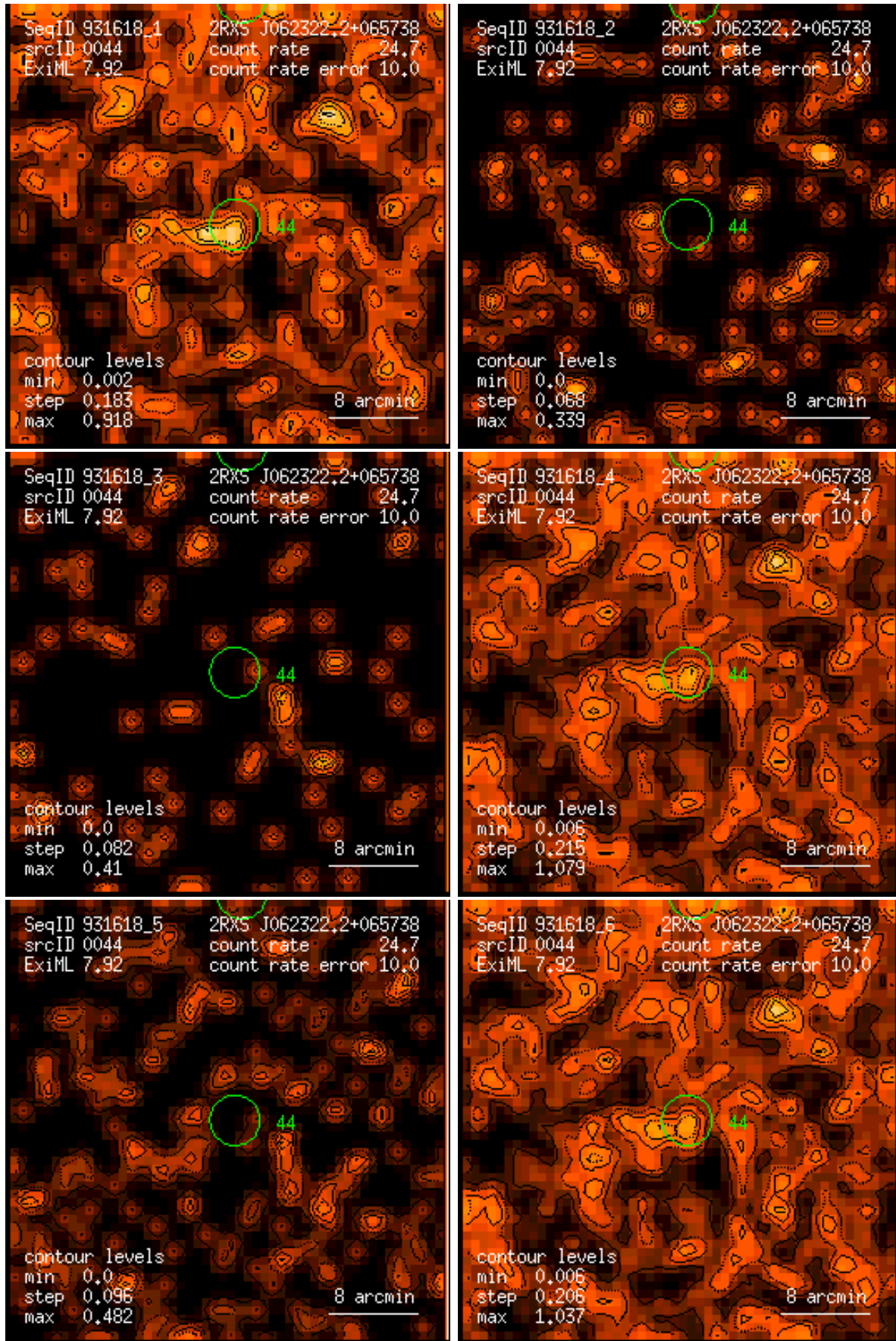
Figure 44: RASS 931618: detection 0044: band rate images, Gaussian filter: (1) PSPC channels 11 – 41, (2) 52 – 90, (3) 91 – 201, (4) 11 – 235, (5) 52 – 201, (6) 11 – 201. Broad band rates in counts/ks. Band rate contour levels in counts/ks/arcmin 2 .
