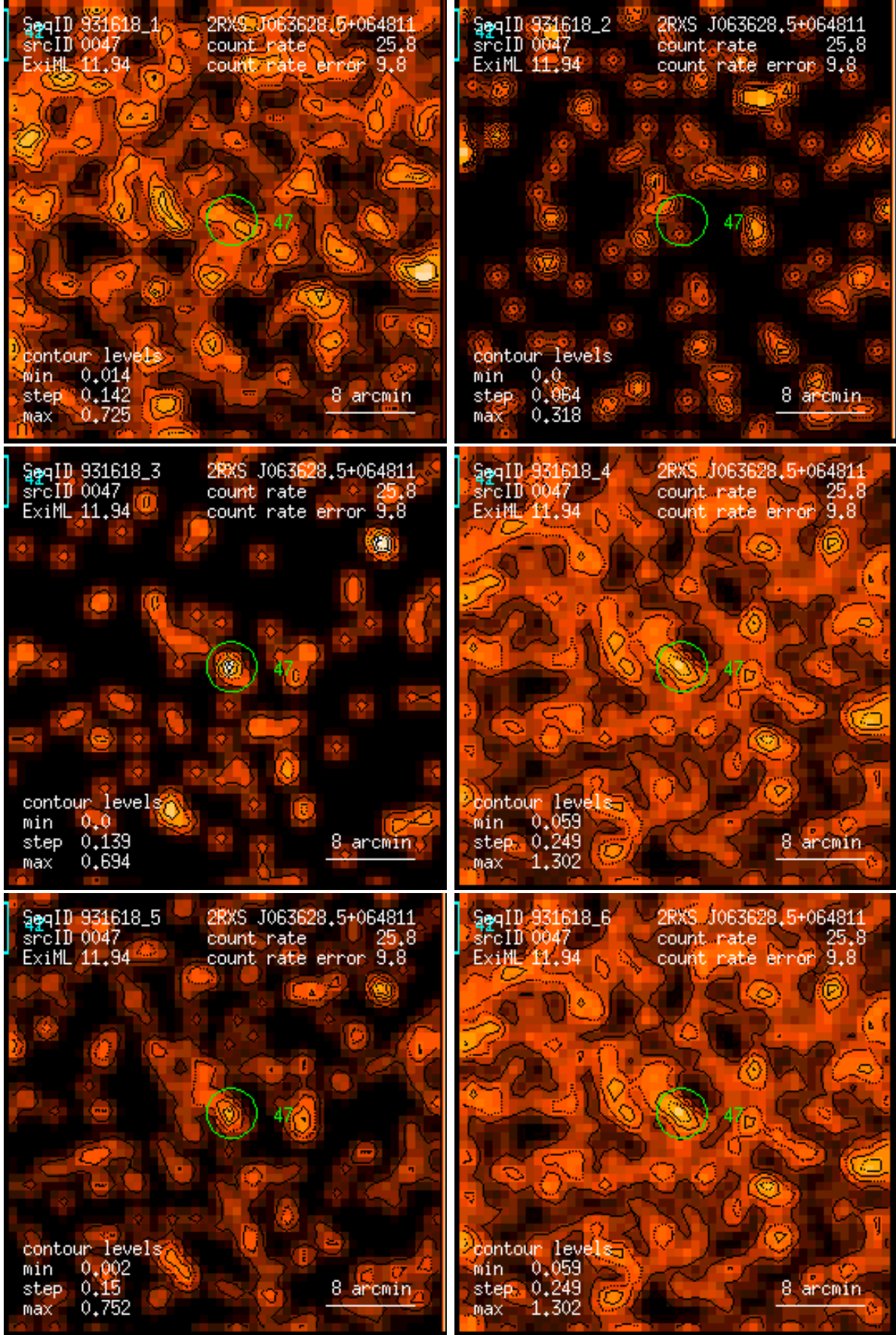
Figure 47: RASS 931618: detection 0047: band rate images, Gaussian filter: (1) PSPC channels 11 – 41, (2) 52 – 90, (3) 91 – 201, (4) 11 – 235, (5) 52 – 201, (6) 11 – 201. Broad band rates in counts/ks. Band rate contour levels in counts/ks/arcmin 2 .
