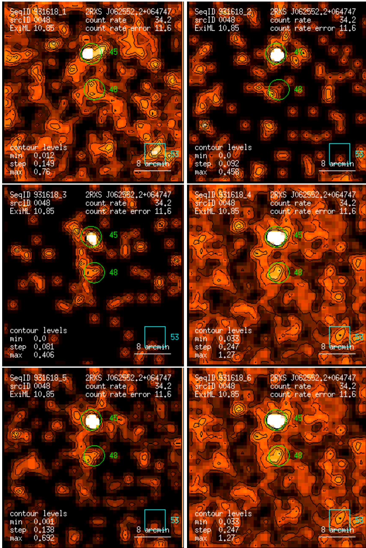
Figure 48: RASS 931618: detection 0048: band rate images, Gaussian filter: (1) PSPC channels 11 – 41, (2) 52 – 90, (3) 91 – 201, (4) 11 – 235, (5) 52 – 201, (6) 11 – 201. Broad band rates in counts/ks. Band rate contour levels in counts/ks/arcmin 2 .
