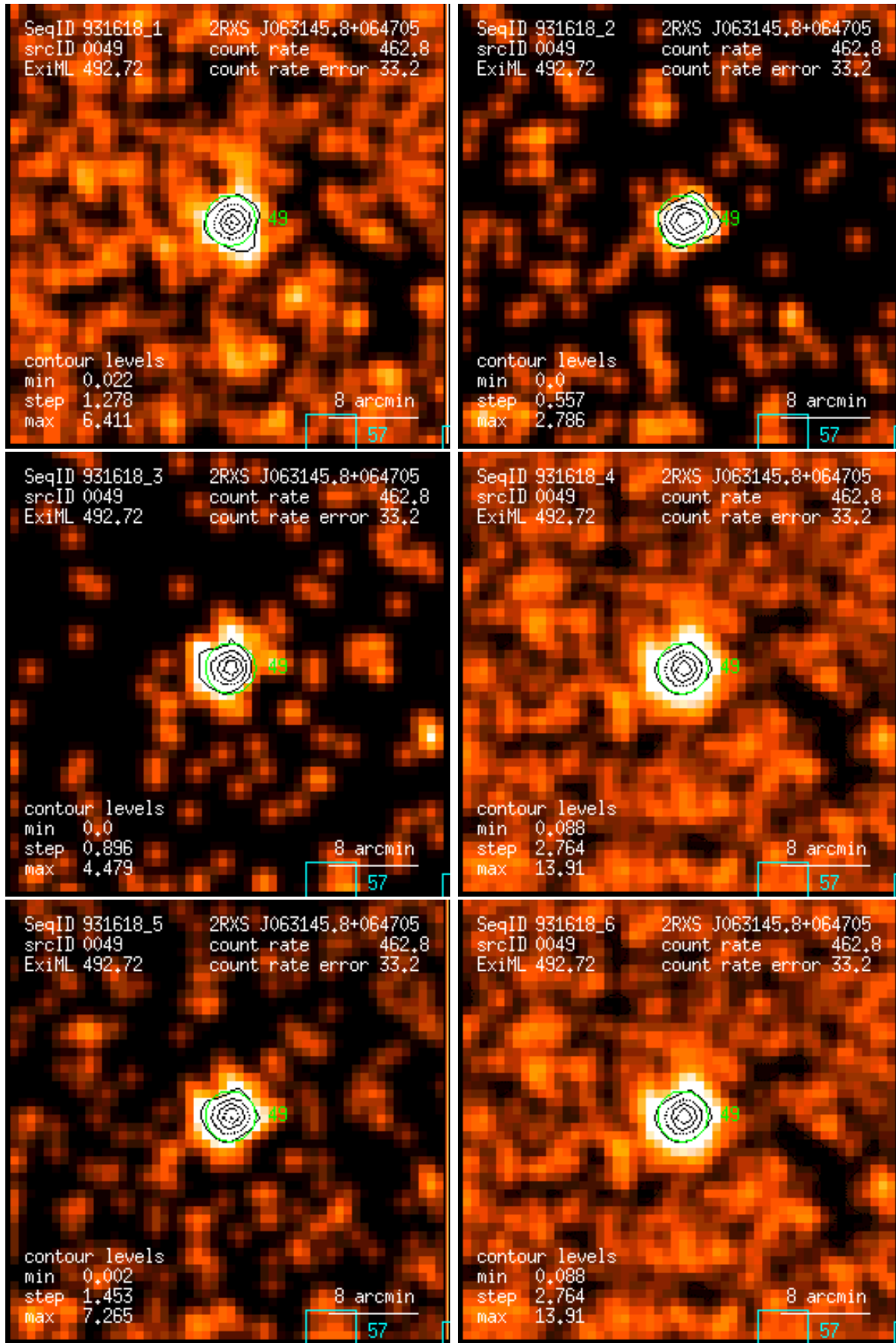
Figure 49: RASS 931618: detection 0049: band rate images, Gaussian filter: (1) PSPC channels 11 – 41, (2) 52 – 90, (3) 91 – 201, (4) 11 – 235, (5) 52 – 201, (6) 11 – 201. Broad band rates in counts/ks. Band rate contour levels in counts/ks/arcmin 2 .
