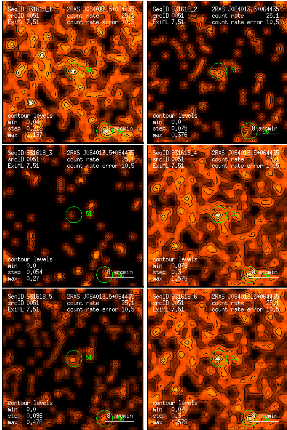
Figure 51: RASS 931618: detection 0051: band rate images, Gaussian filter: (1) PSPC channels 11 – 41, (2) 52 – 90, (3) 91 – 201, (4) 11 – 235, (5) 52 – 201, (6) 11 – 201. Broad band rates in counts/ks. Band rate contour levels in counts/ks/arcmin 2 .
