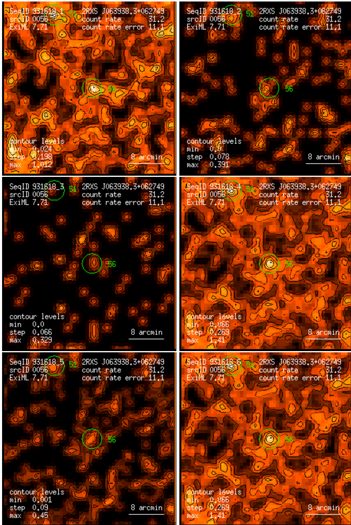
Figure 56: RASS 931618: detection 0056: band rate images, Gaussian filter: (1) PSPC channels 11 – 41, (2) 52 – 90, (3) 91 – 201, (4) 11 – 235, (5) 52 – 201, (6) 11 – 201. Broad band rates in counts/ks. Band rate contour levels in counts/ks/arcmin 2 .
