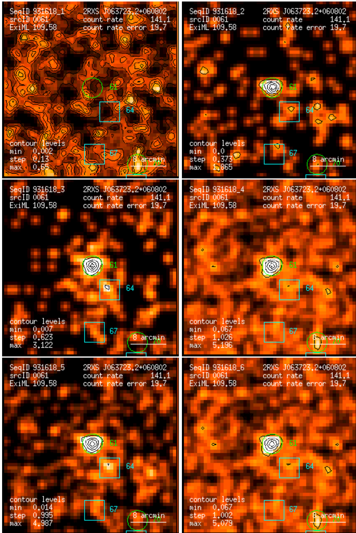
Figure 61: RASS 931618: detection 0061: band rate images, Gaussian filter: (1) PSPC channels 11 – 41, (2) 52 – 90, (3) 91 – 201, (4) 11 – 235, (5) 52 – 201, (6) 11 – 201. Broad band rates in counts/ks. Band rate contour levels in counts/ks/arcmin 2 .
